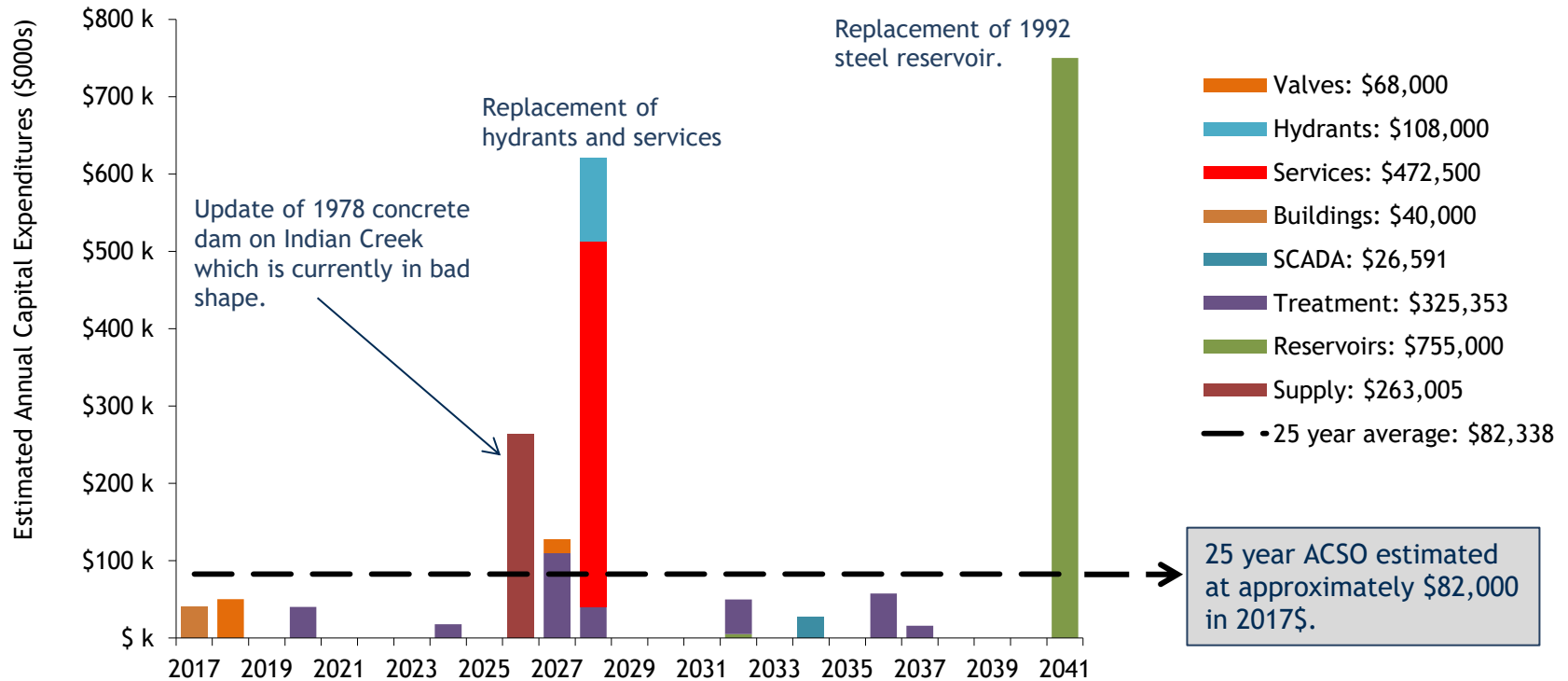
Figure 5: Riondel 25 Year Asset Replacement Schedule
