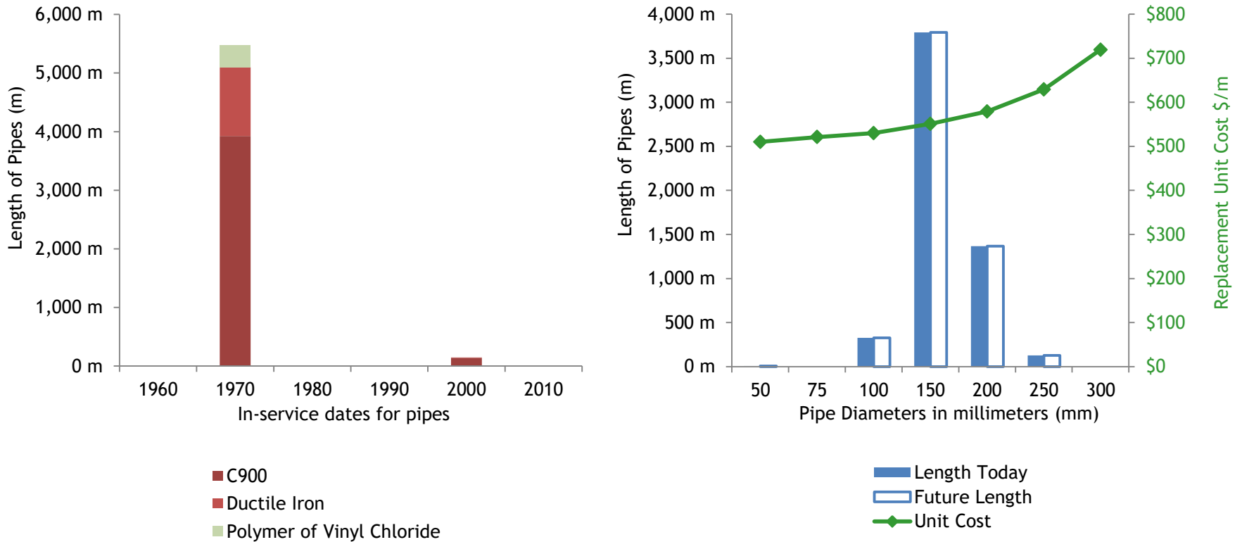
Figure 2: Riondel Pipe Distribution Network (Length, Material, Diameter)
