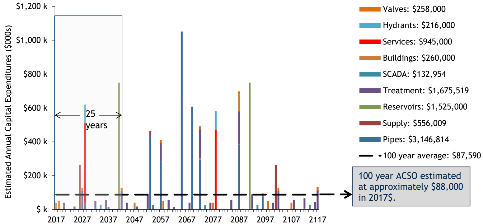
Figure 6: Riondel 100 Year Asset Replacement Schedule
