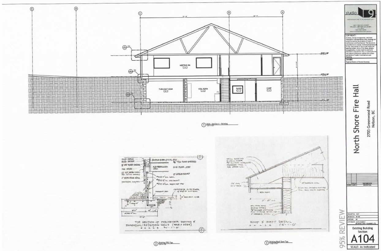
CROSS SECTION
