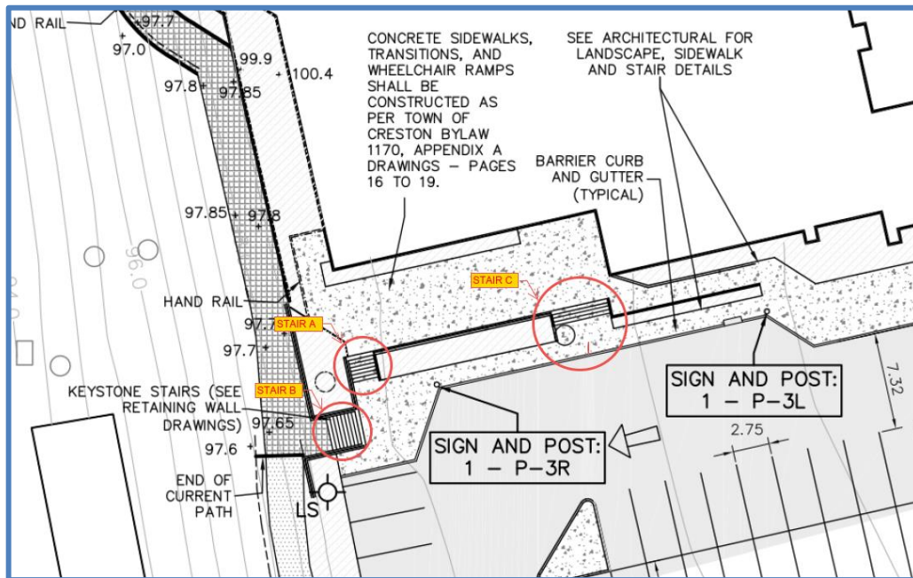
Figure 1 - Excerpt from "2010-06-04-Creston_Civil_Surface_Works-Drawing"
