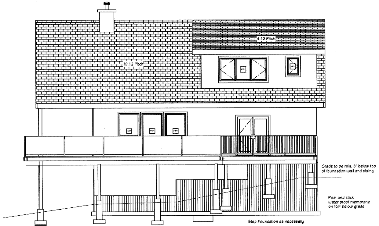
South Elevation
