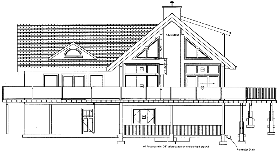
West Elevation
