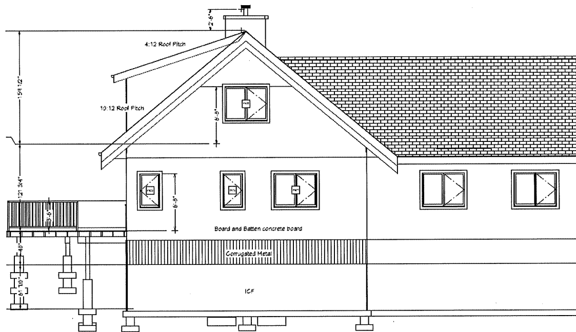
East Elevation
