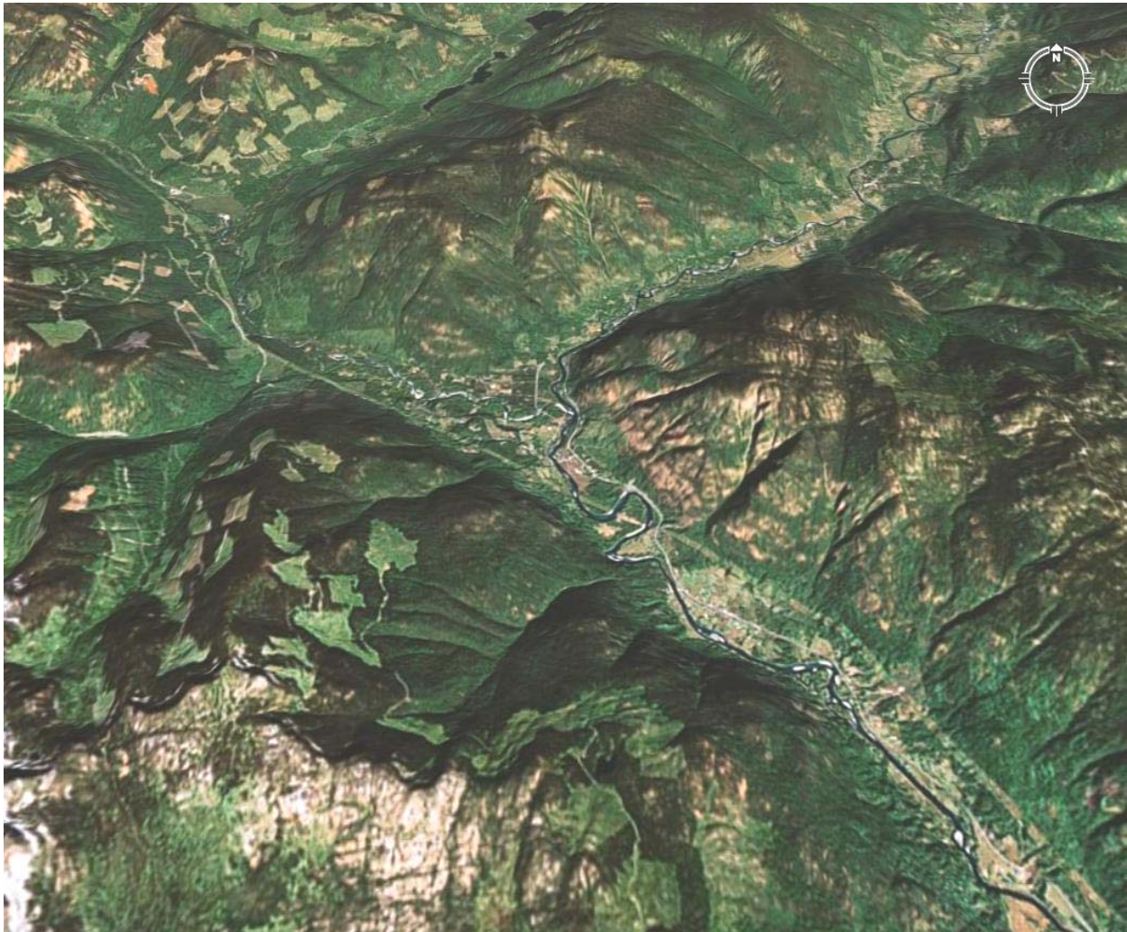
Figure 1. View of topographic relief of the Passmore Fire Protection Area looking north (sourced from Google Earth™, 2007).
